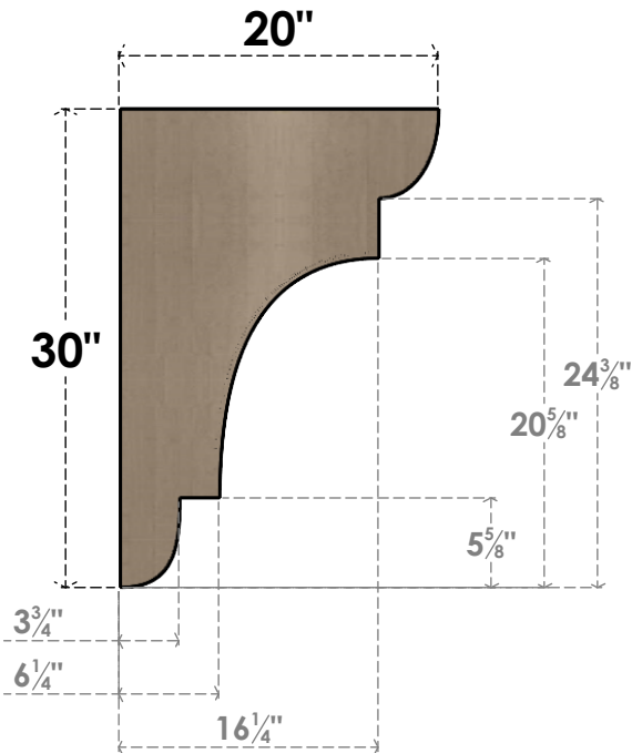
SIDE PROFILE
