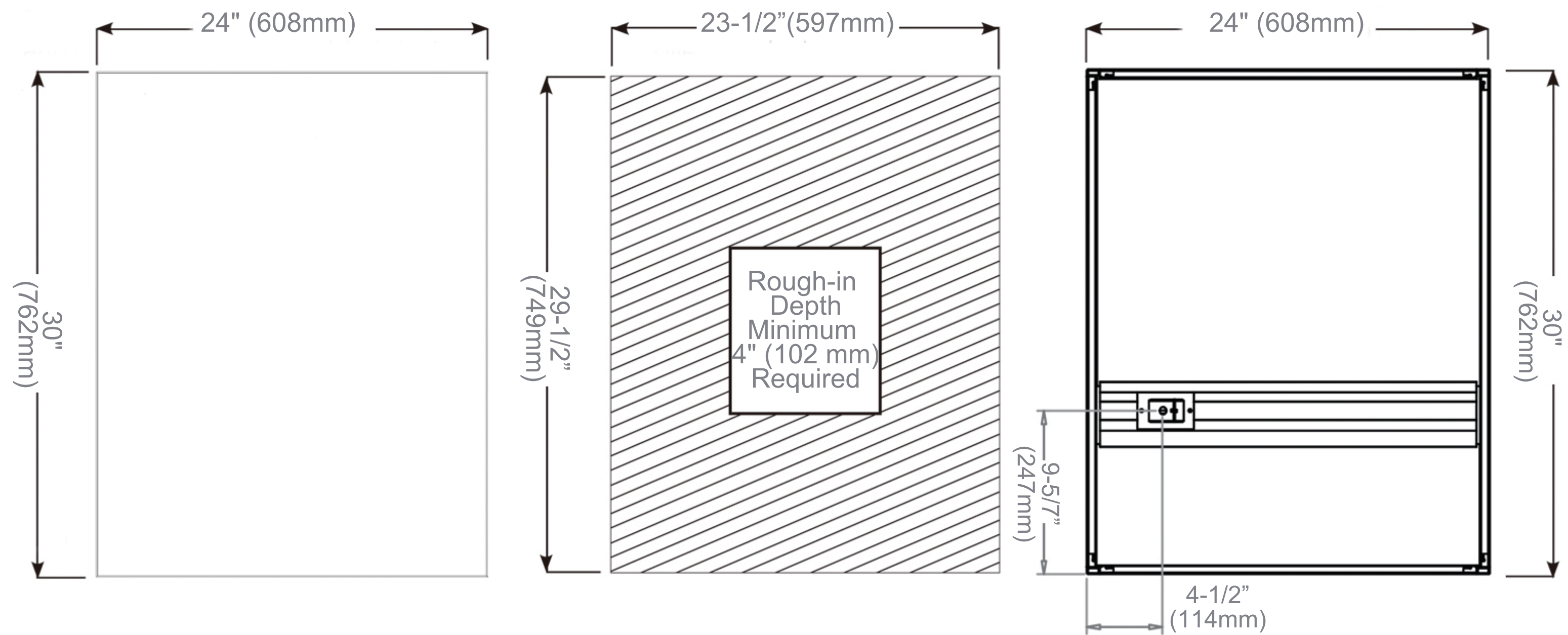
Cabinet Dimensions
