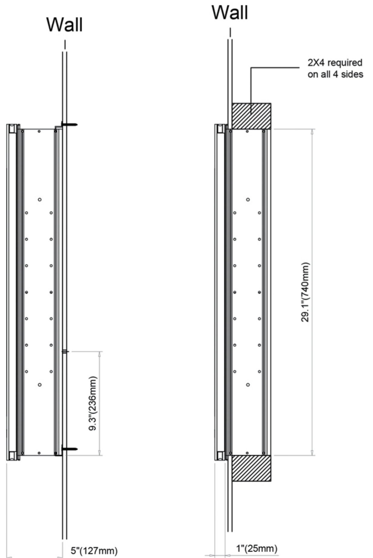
Recessed Mount
