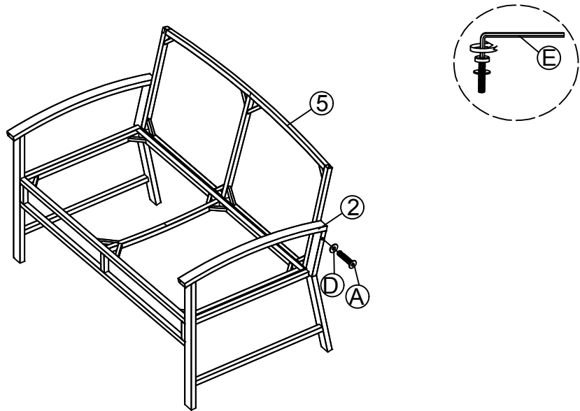
STEP 9: Connect The Part from Step (8) & Left Frame (2), tighten Allen Bolt (A), Flat Washer (D) with Allen Key (E).
