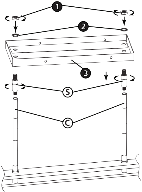
{ DRAWING 1- INSTALLATION }
