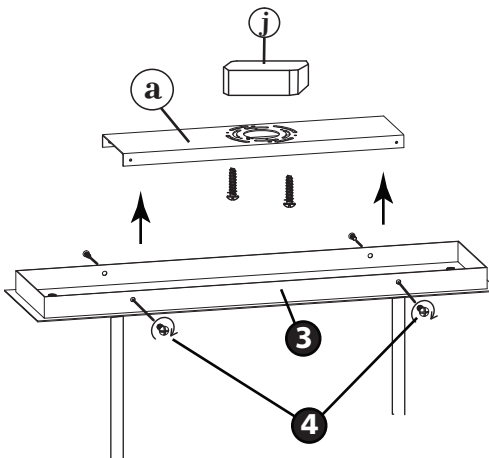
{ DRAWING 2 - INSTALLATION }
