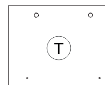
TR2319 292x357x18mm
