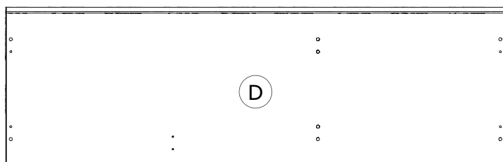
BA2248 1282x404x22mm
