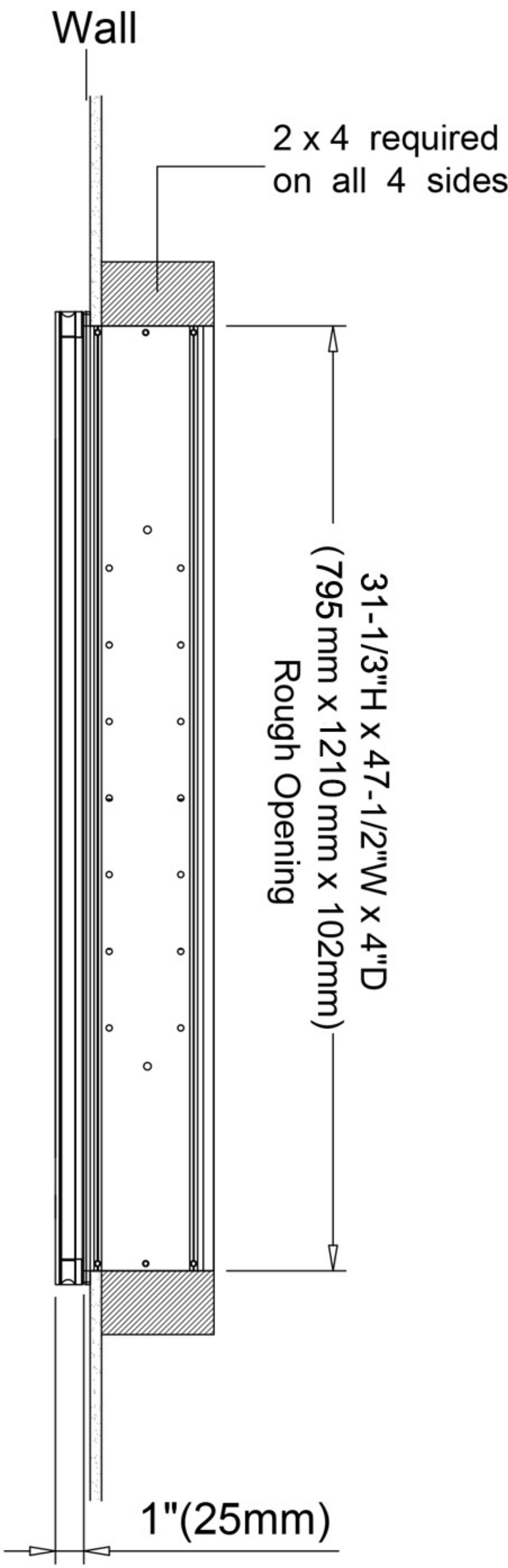
Recessed Mount
