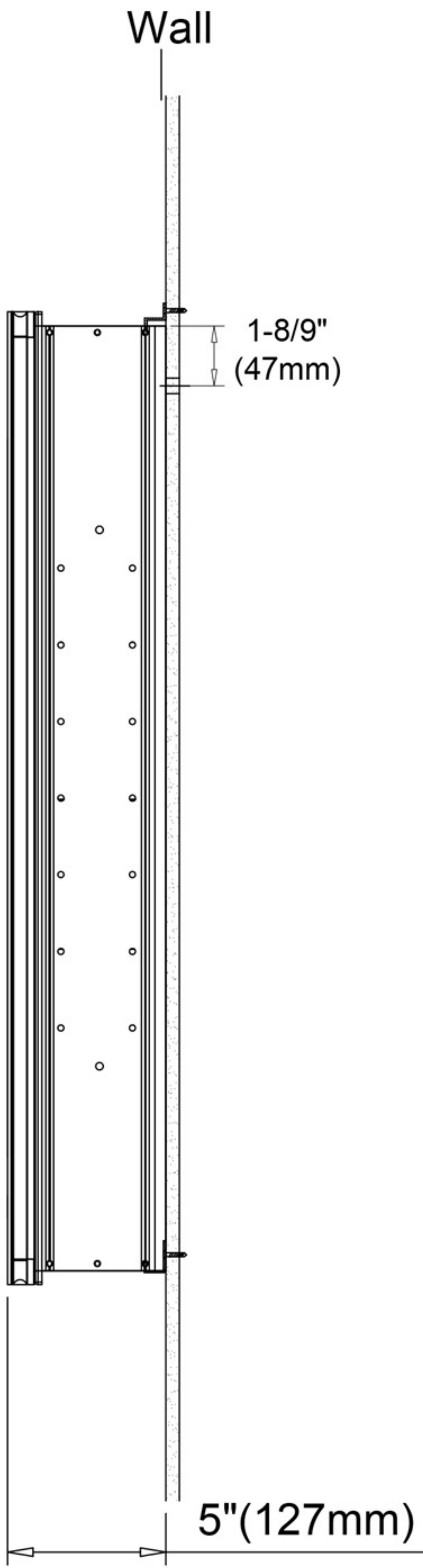
Surface Mount
