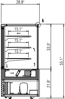
SECTION VIEW
