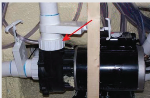
FIGURE 1.5B -- PUMP UNION; LOOSEN UP TO BLEED AIR
