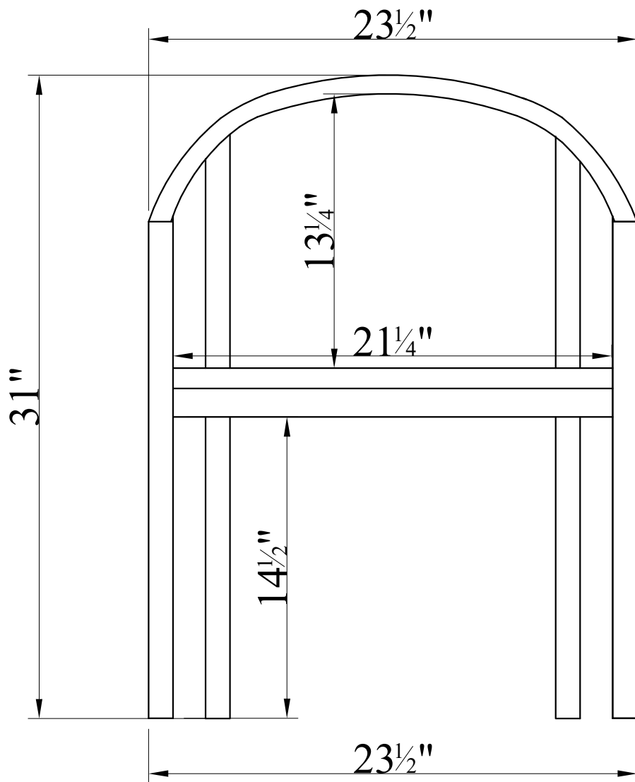
FRONT VIEW
