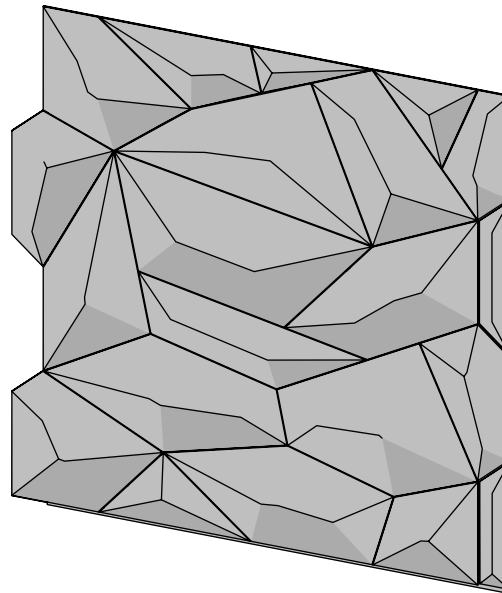
GLACIER
