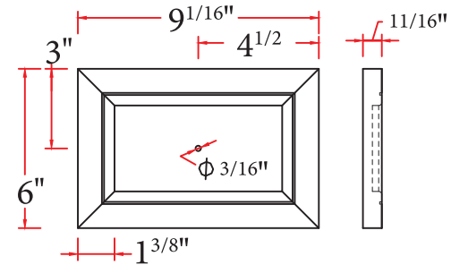
— SMALL DRAWER —
