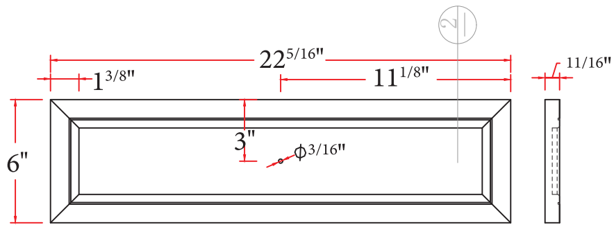
— LARGE DRAWER —
