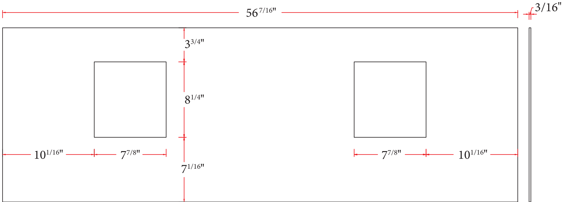
— BACKBOARD —
