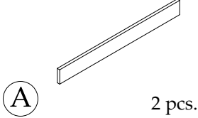
File Bar
