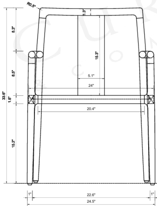
FRONT VIEW
