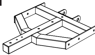
seat support - 1 pc
