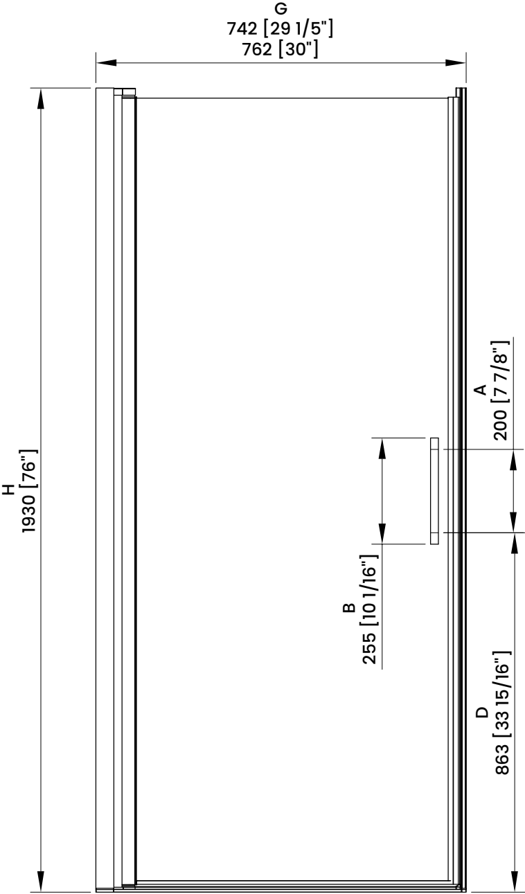
Measurements provided are in mm and inches.
