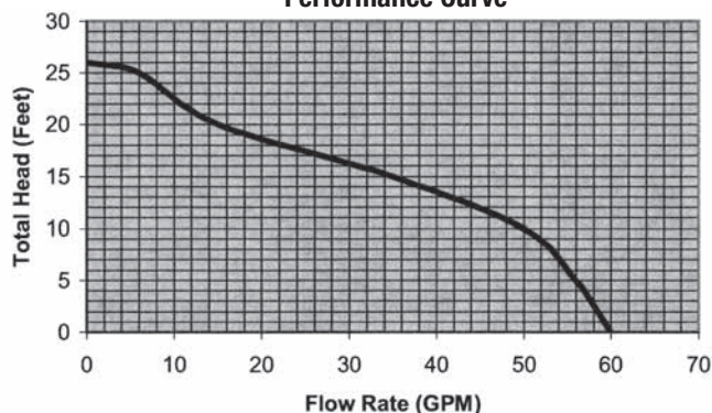
Performance Curve
