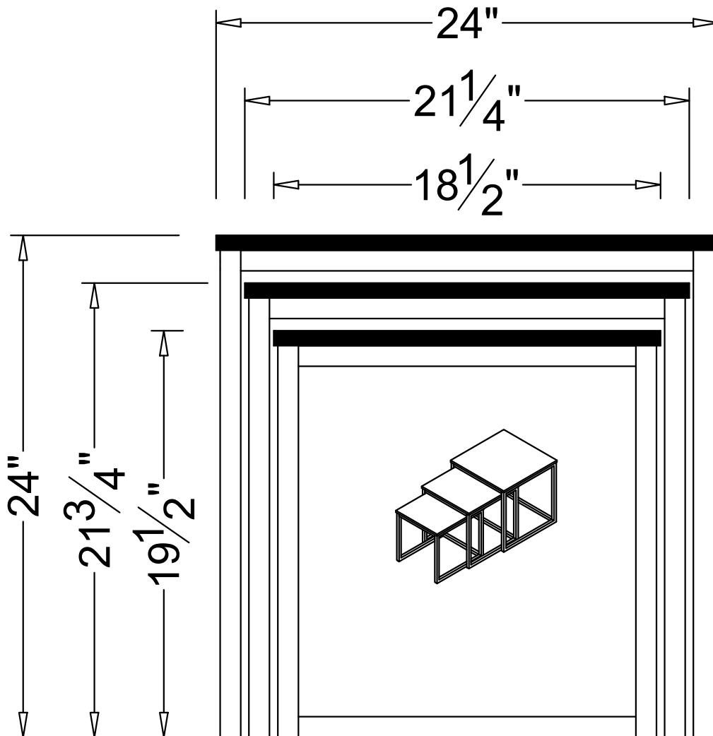
FRONT VIEW
