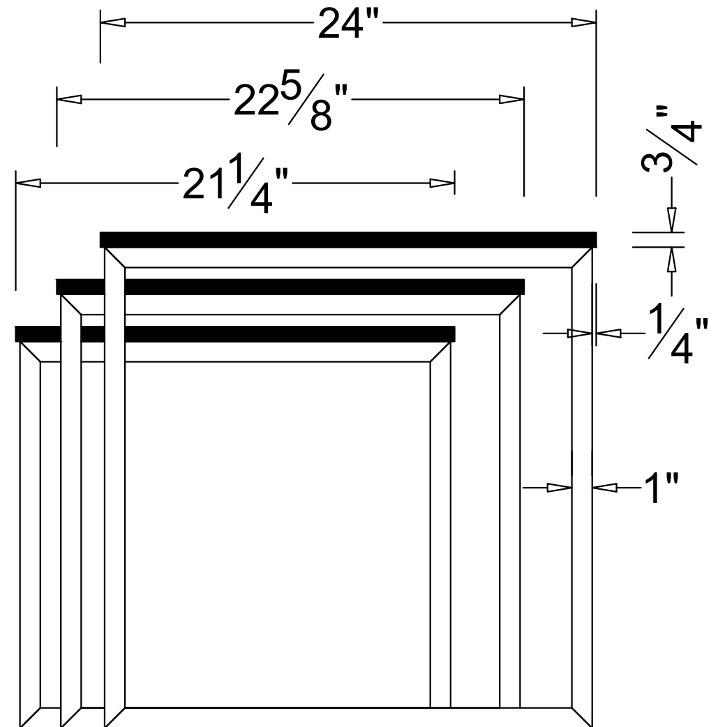
SIDE VIEW
