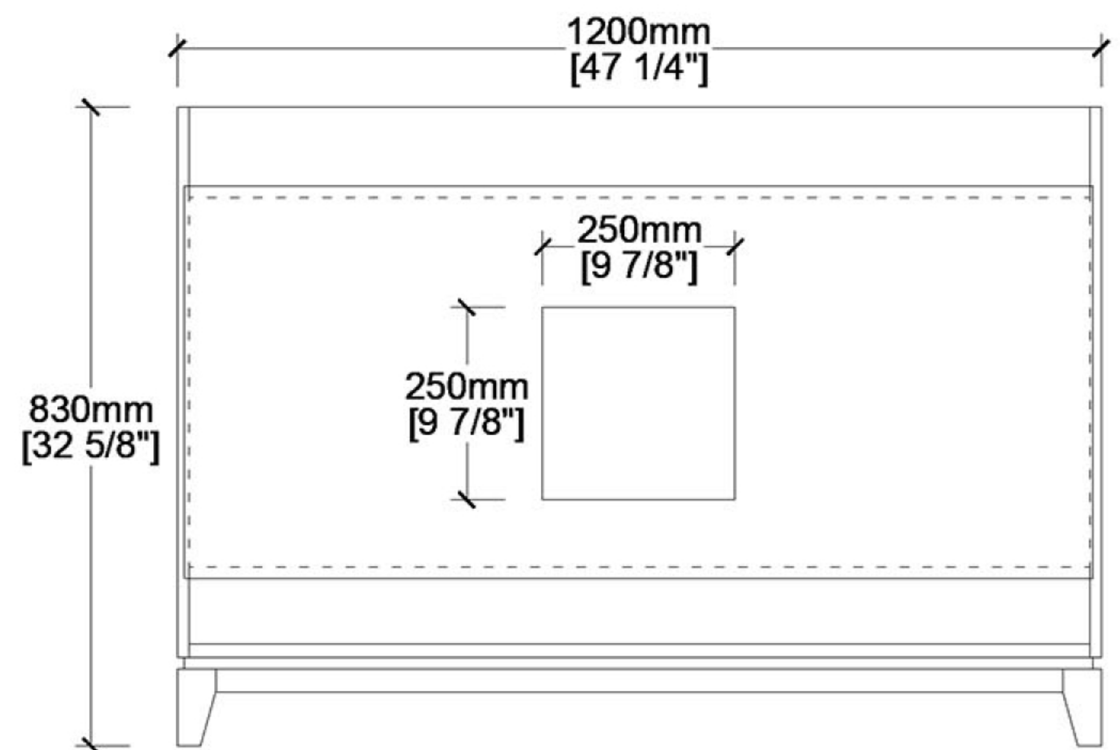
BACK VIEW
