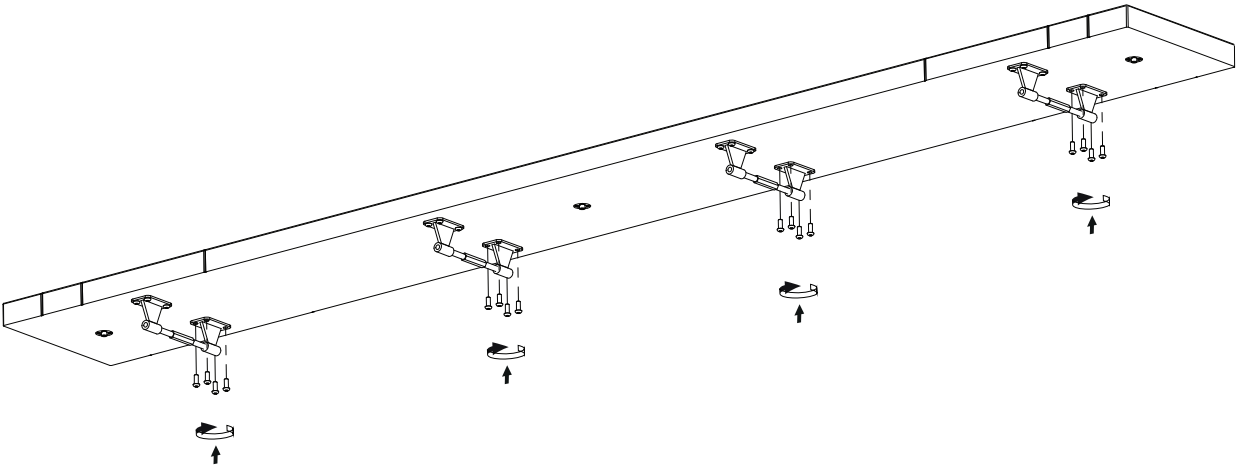
BOTTOM VIEW
