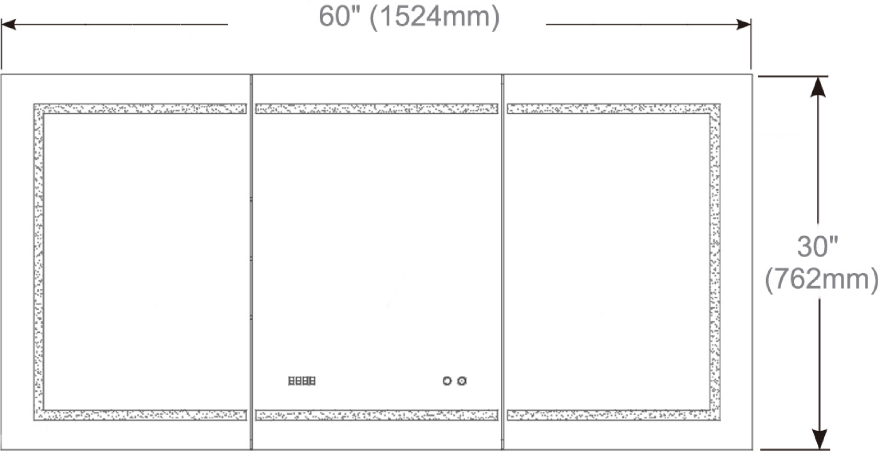
Cabinet Dimensions
