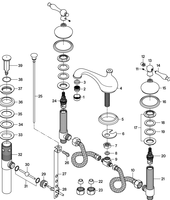
Hot Cartridge: KSRPL5000HC
