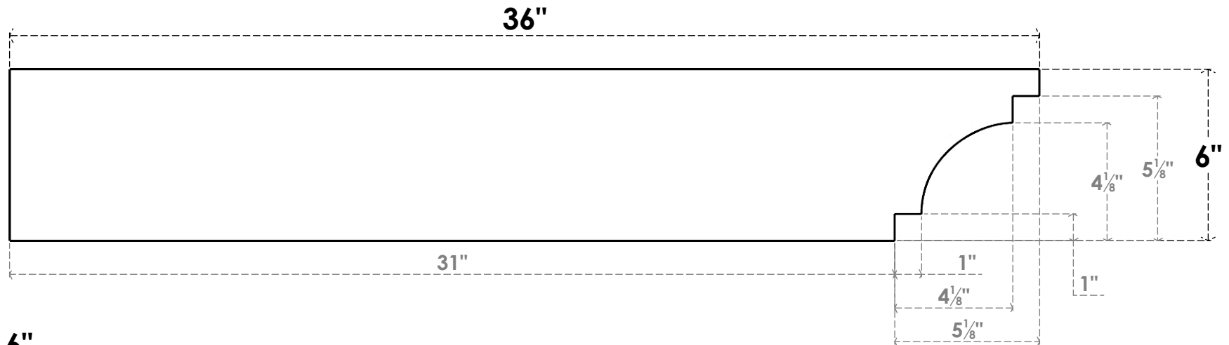
SIDE PROFILE
