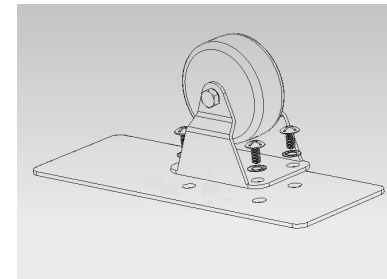
Fixed wheels
