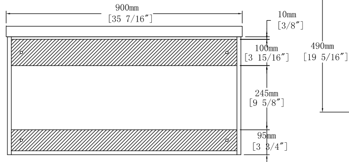
Back View
