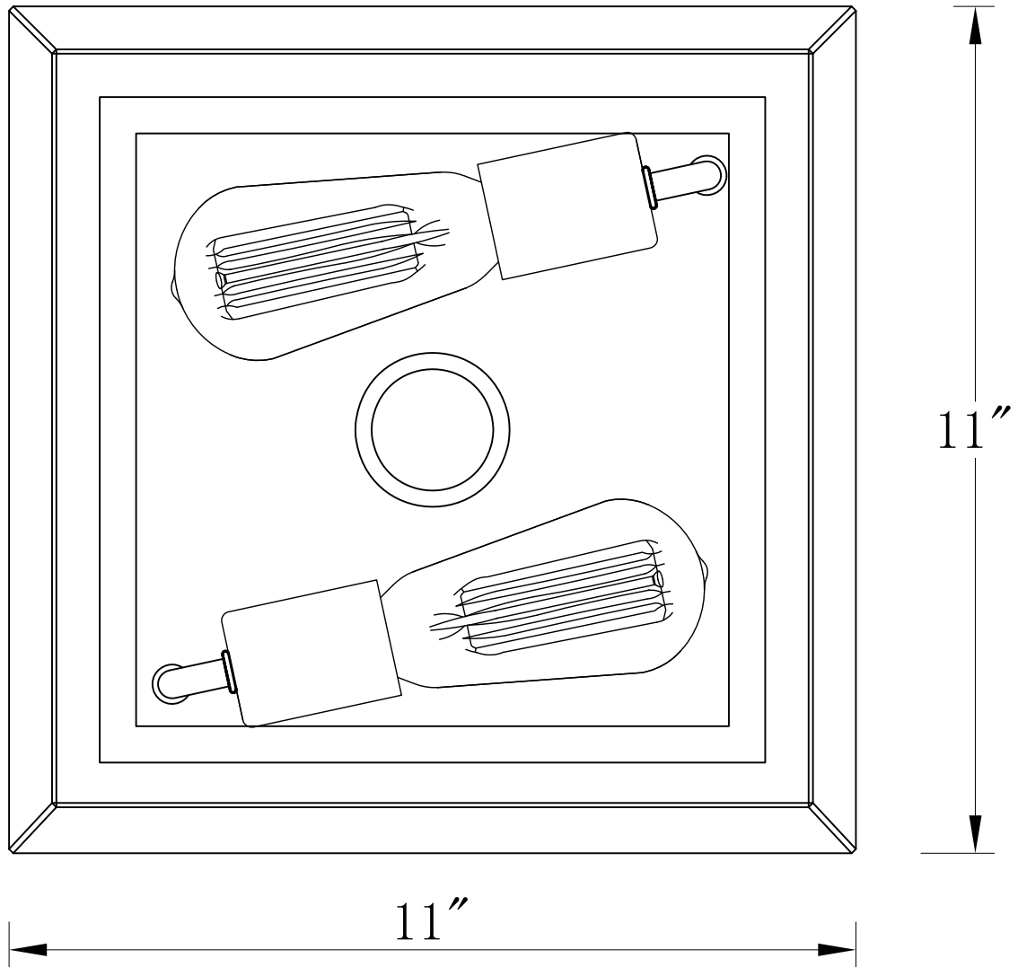
TOP VIEW
