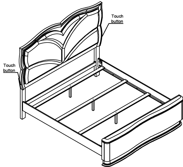
Assembly Completed
