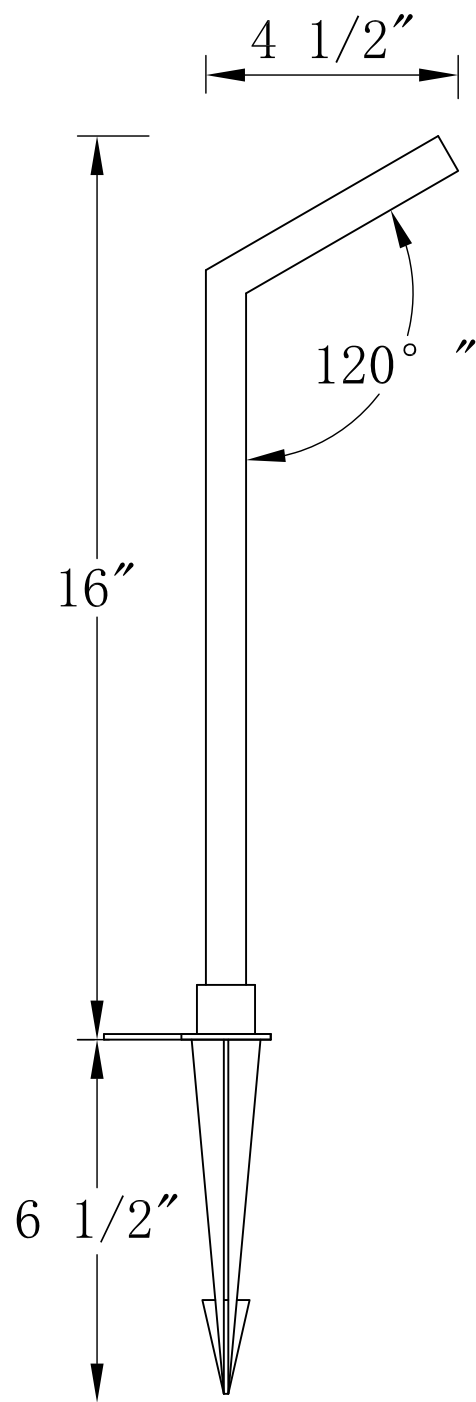
FRONT VIEW
