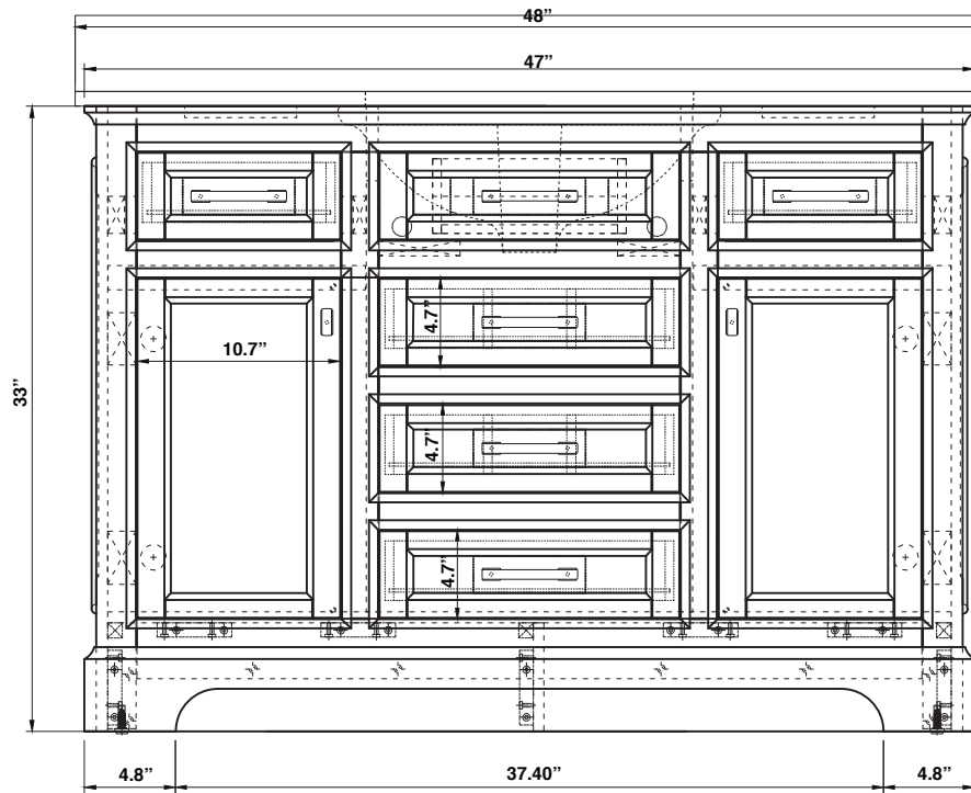
(Front View)
