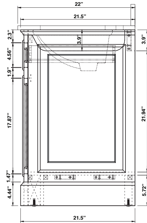
(Side View)
