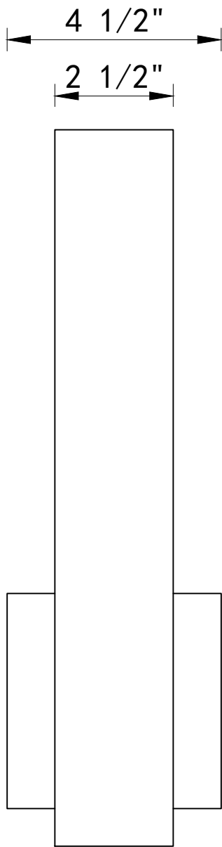
FRONT VIEW
