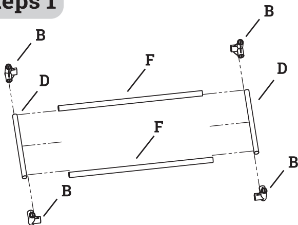
Assemble B and D
