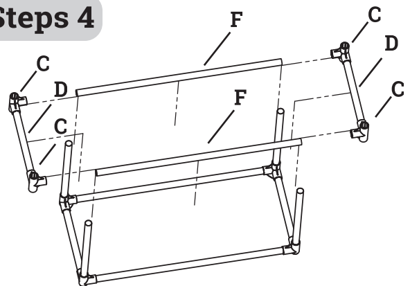
Assemble C and D first, then assemble F
