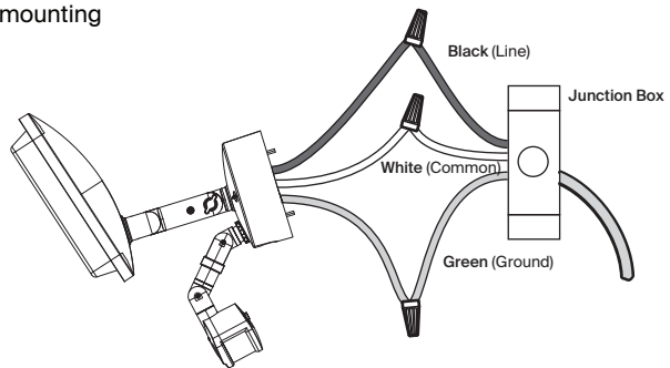
Non-Dimming Wiring Diagram
