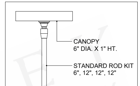
CANOPY DETAIL
