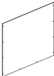
17 (490*400*3mm x2)
