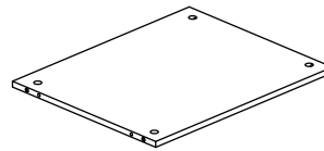
7 (469*380*12mm x2)
