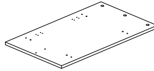
3 (676*397*15mm x1)
