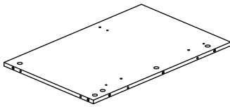
5 (586*381*12mm x1)
