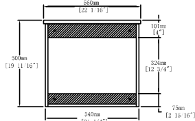
Back View
