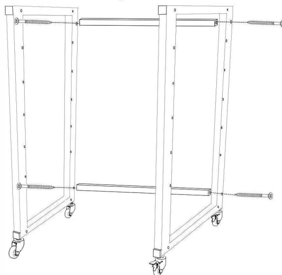
Second-Assemble 2 Pipe
