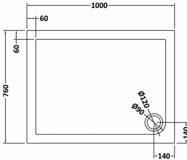
1000 x 760 RECTANGULAR TRAY
