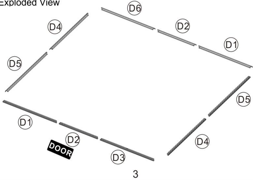
Base Exploded View
