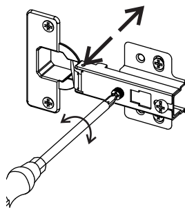
Lateral adjustment
