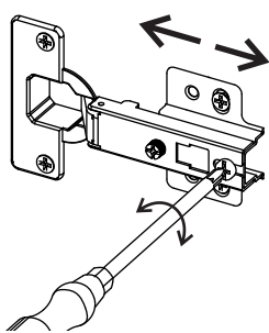
Depth adjustment
