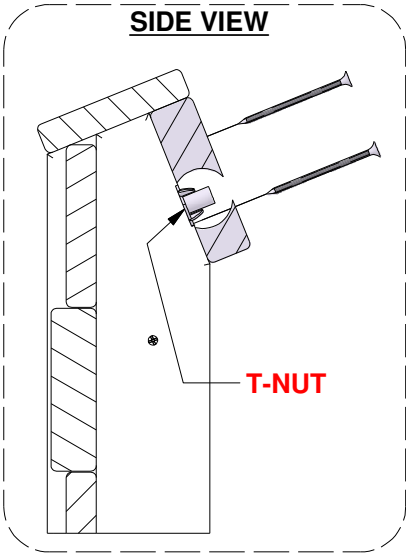
090 (x8) SCREW - 2 1/2"
