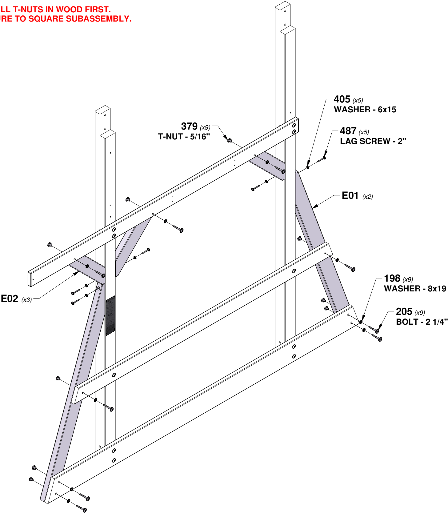
E02 DECK BRACE - W4L16598 (x3) 1 3/8"x3 3/8"x17" (36x86x433)
