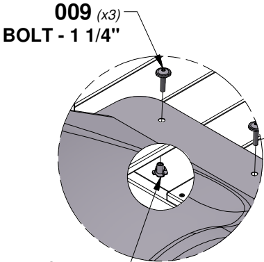
074 (x3) T-NUT - 5/16"
