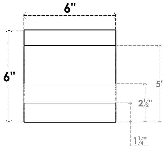
FRONT PROFILE
