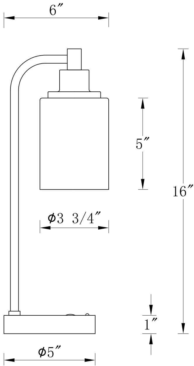
FRONT VIEW
