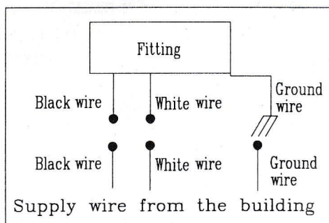
Circuit diagram 1
