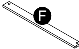
Support (x4) 39100222060
