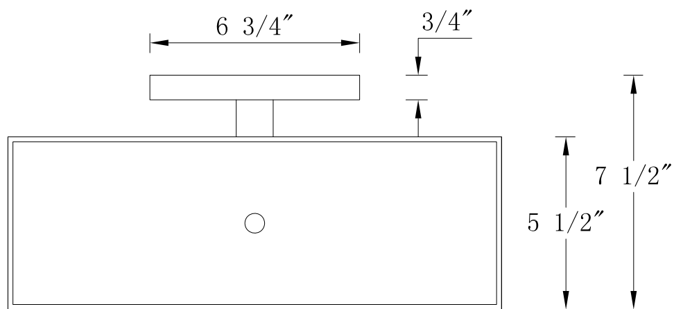
TOP VIEW
