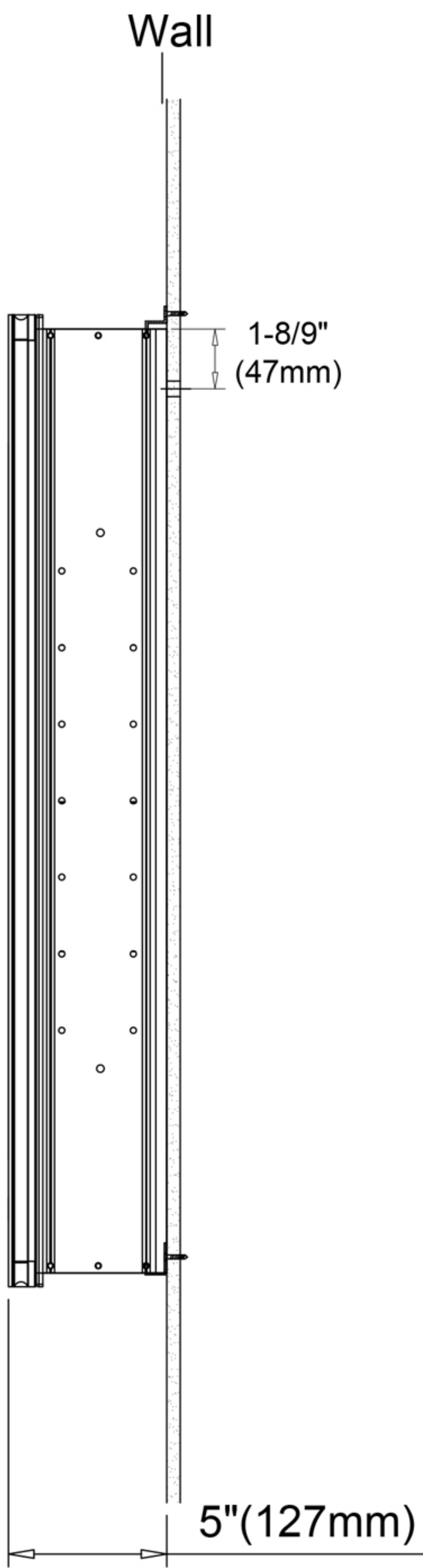
Surface Mount
