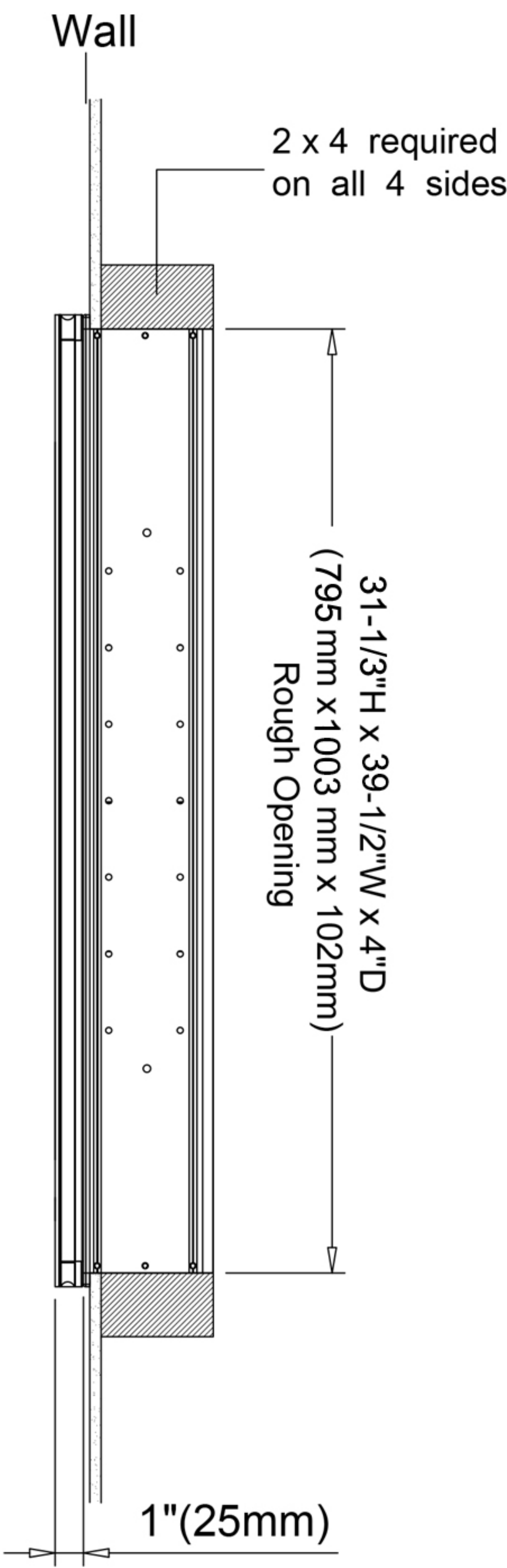
Recessed Mount
