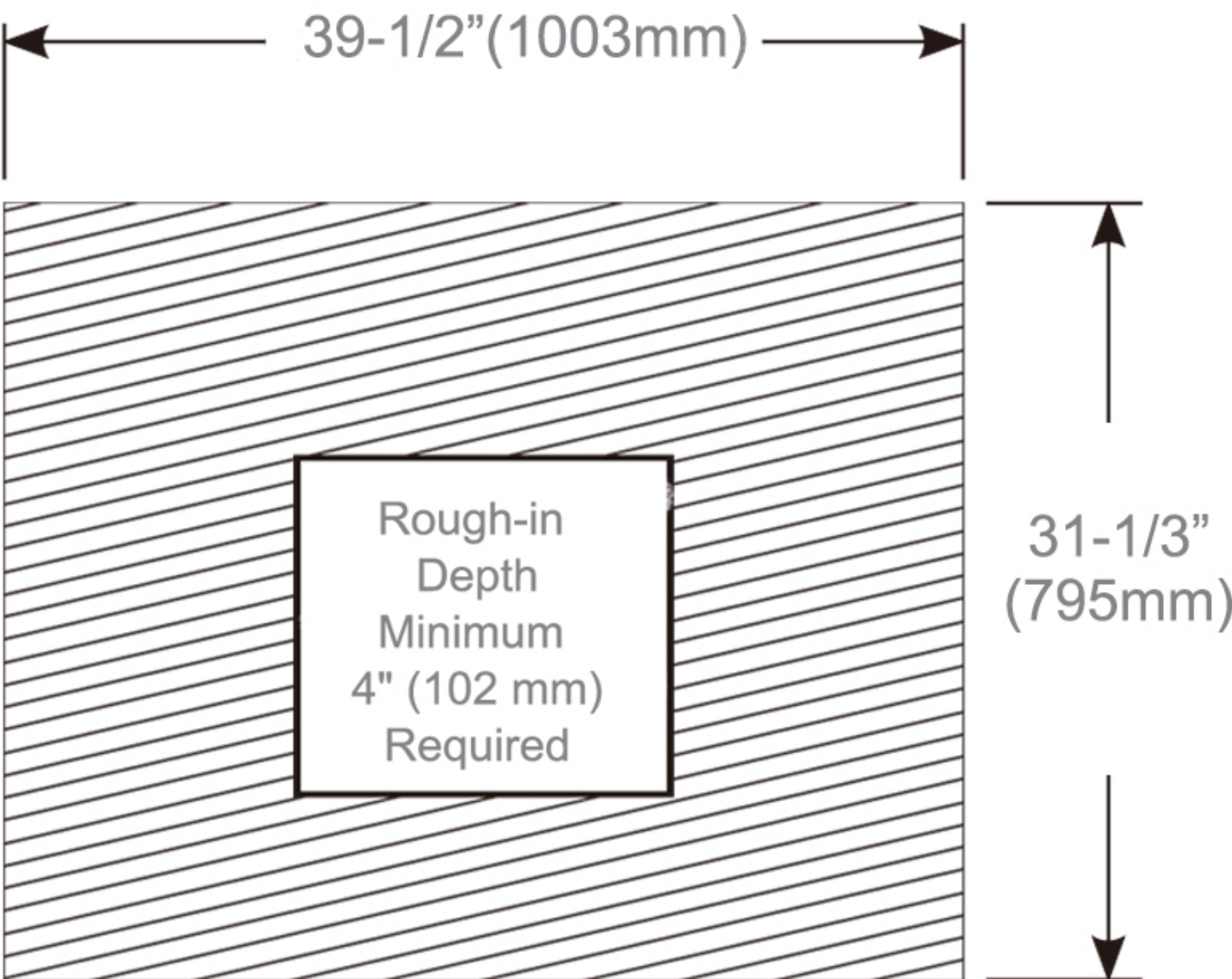
Rough-in Dimensions
