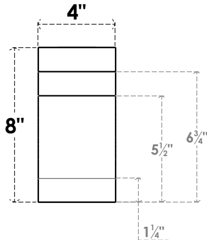
FRONT PROFILE
