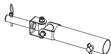
Landmine Attachment - 1 pc
