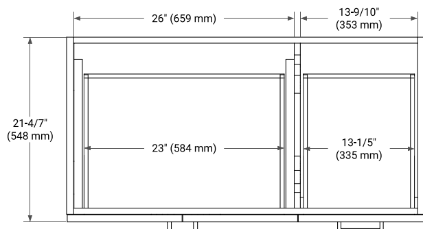
PLAN VIEW
