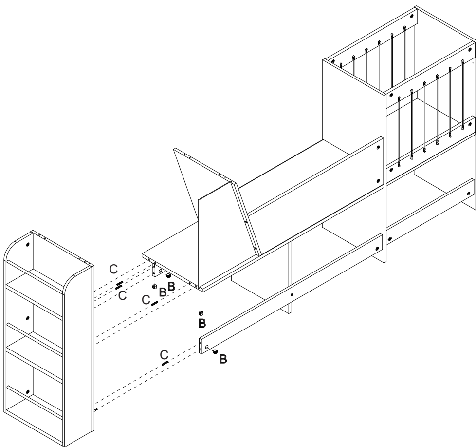
Cam Lock Fastening System
