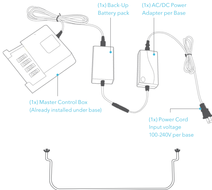
(1x) Foot Retainer bar (2x) Wing-nuts per Base
