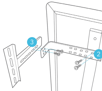
(4x) Under Bracket
